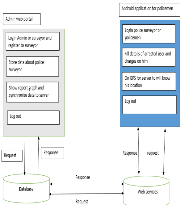
Fig. 1 Architecture diagram for application
