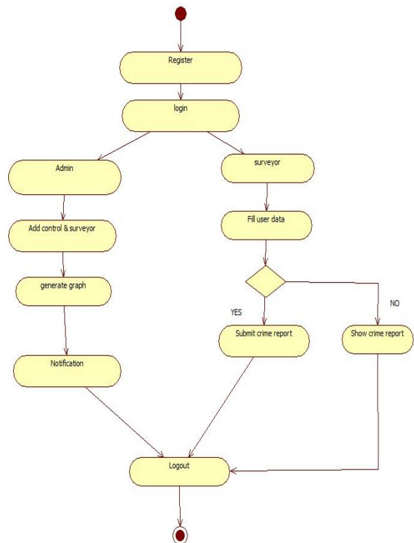
Fig. 2. Activity Diagram
